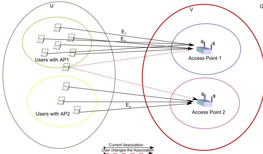
Fig. 3. Bigraph represents the example
